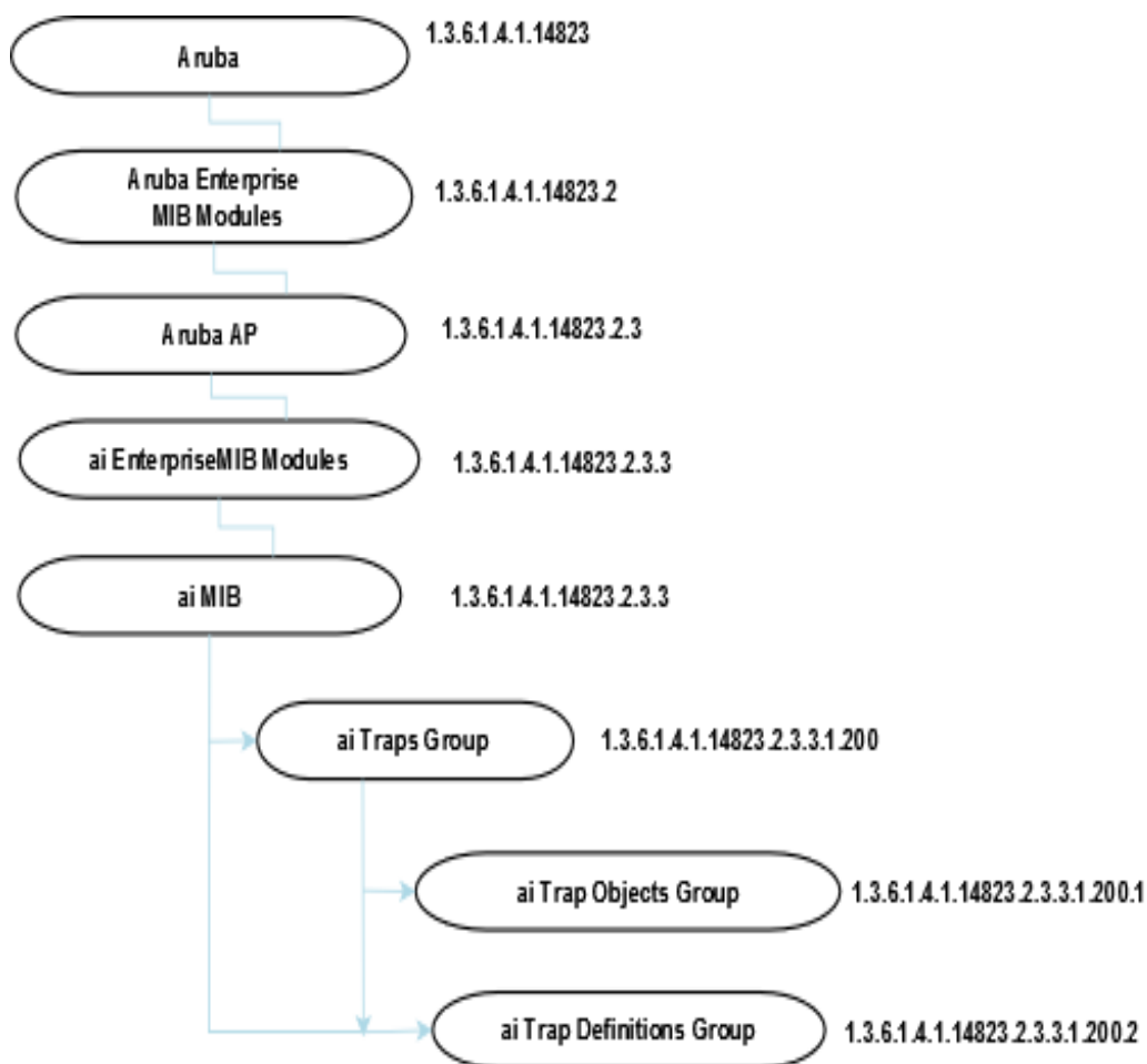
Figure 5 Trap Hierarchy
